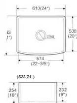
Apron Kitchen Sink Embedded Type Size: 610x533x254 mm 24"x21"x10"
