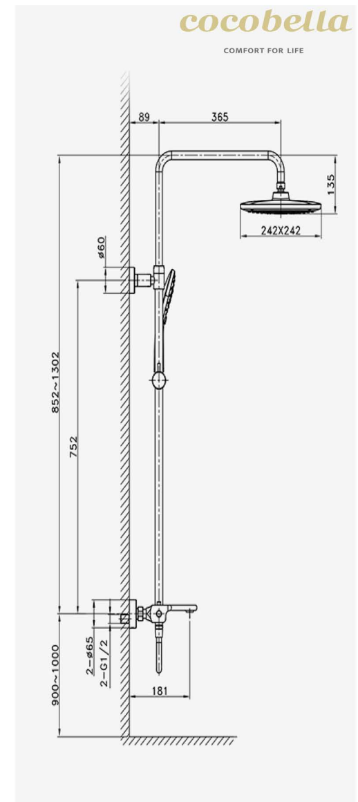
CB.10.98191A-3 Thermostatic rain shower faucet(10" ABS head)
