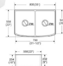
Apron Kitchen Sink Embedded Type Size: 835x558x254 mm 33"x22"x10"
