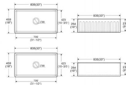
Apron Kitchen Sink Embedded Type Size: 835x459x254 mm 33"x18"x10"
