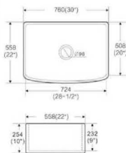
Apron Kitchen Sink Embedded Type Size: 760x558x254 mm 30"x22"x10"
