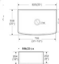
Apron Kitchen Sink Embedded Type Size: 835x558x254 mm 33"x22"x10"
