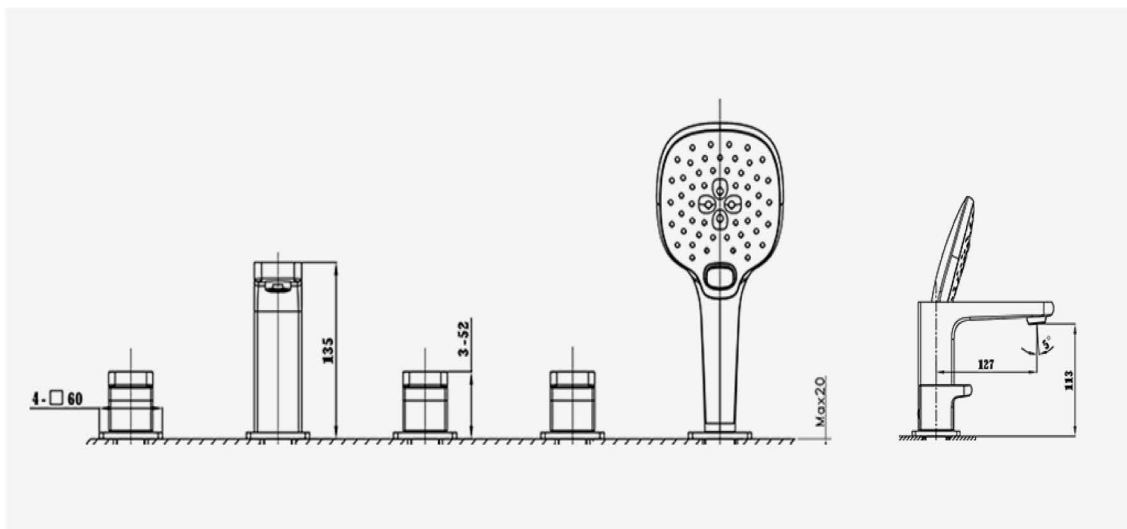
CB.18.983902-07 5-Hole Bath faucet
